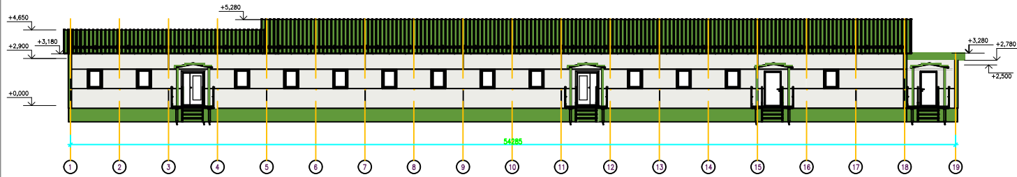
Facade 1-19
