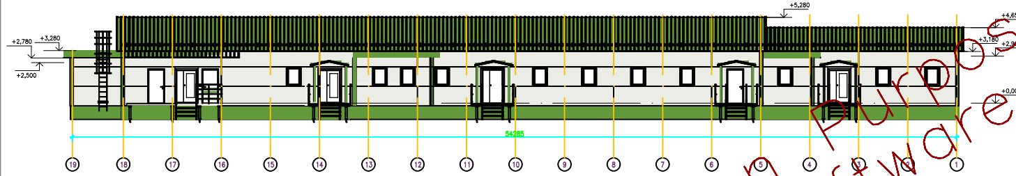
Facade 19-1
