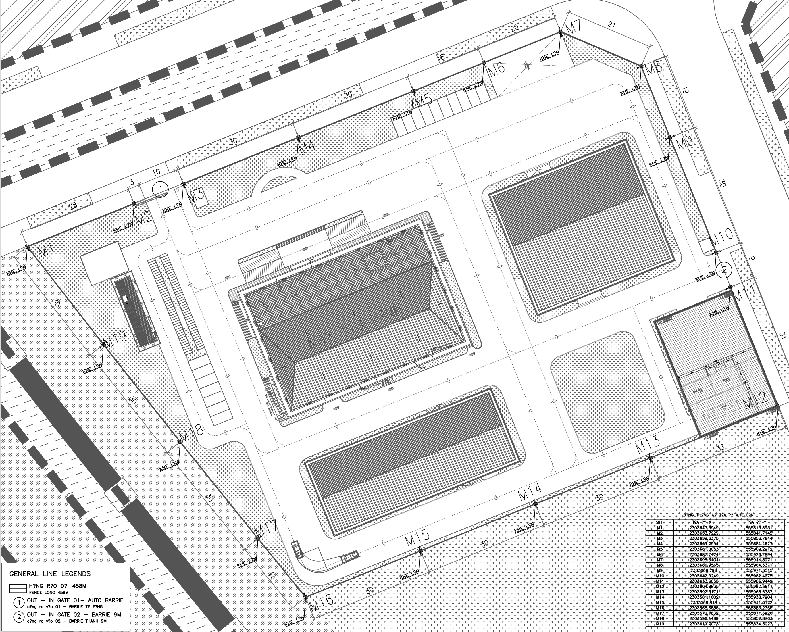
PLAN (M?T B?NG) MASTER PLAN OF GATE- FENCE (T?NG M?T B?NG C?NG H?NG R?)
