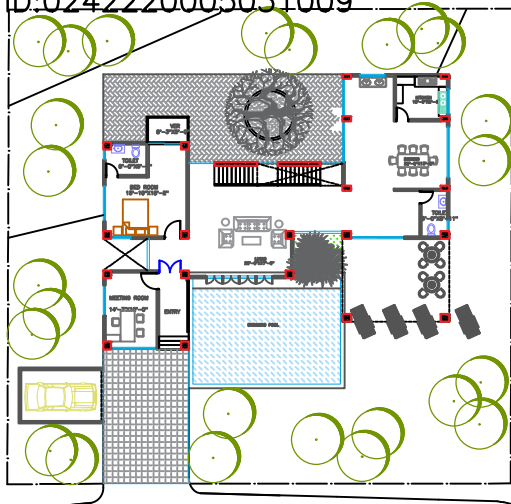
GROUND FLOOR SCALE: 1.100
